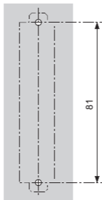
Fig. 5. Drilling plan
